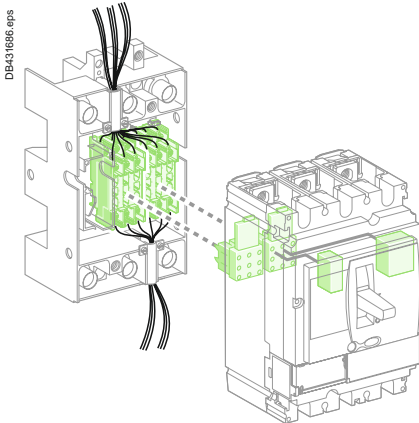
Plug-in/withdrawable Compact NSX DC.
