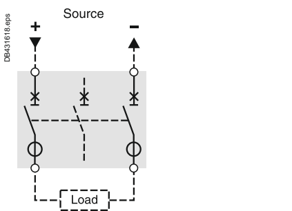
Masterpact NW10N DC version C.
