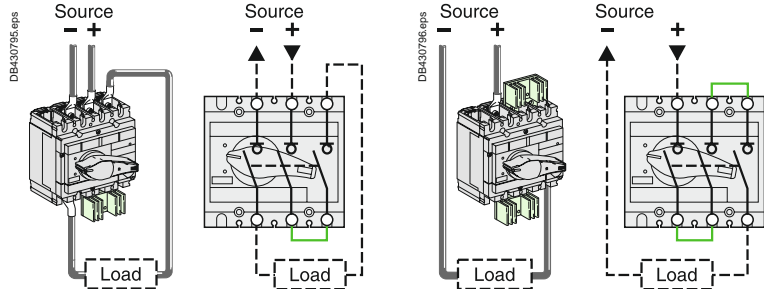
One type of connection per frame size, two catalogue numbers for all series connections.
