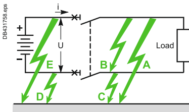
Isolated system.
