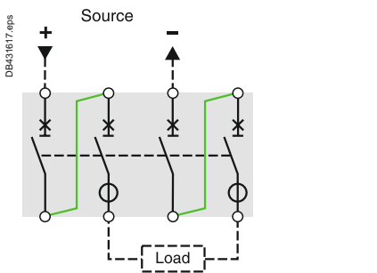
Masterpact NW20H DC version E.
