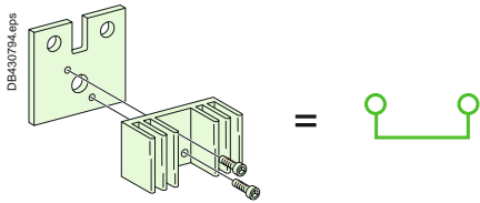
One type of connection per frame size, two catalogue numbers for all series connections.
