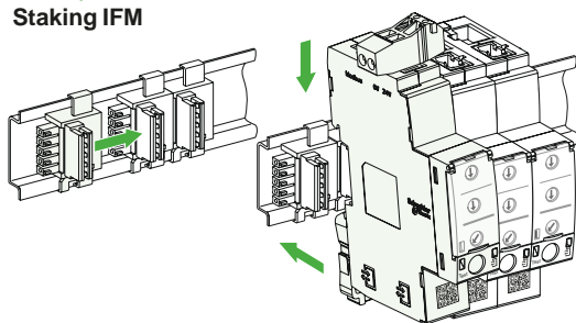
Stacking accessories
