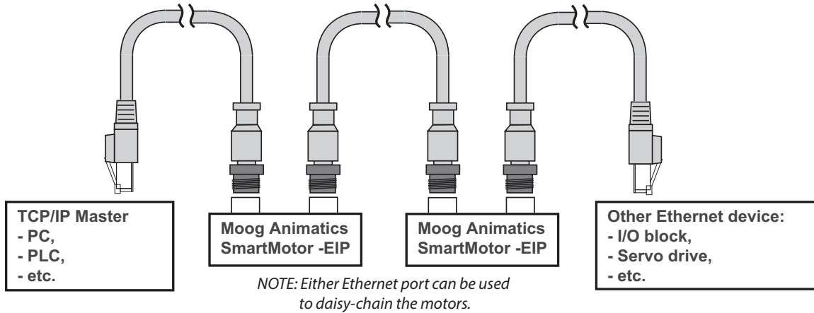
Example Daisy-Chain Configuration
