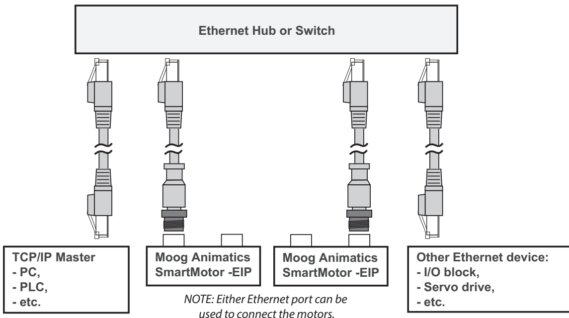
Example Star Configuration
