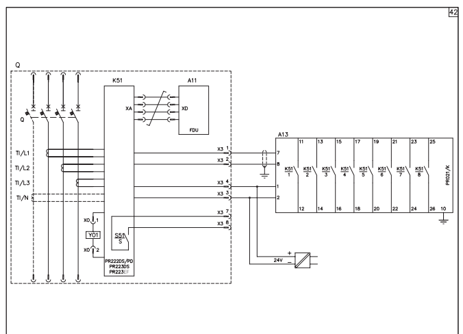
PR222DS/PD和PR223DS或PR223EF电子脱扣器与PR021/K信号单元的连接
