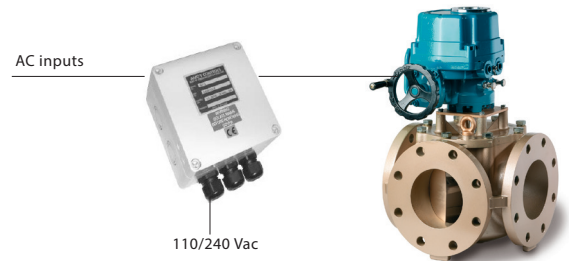
Interface with AC input signals
